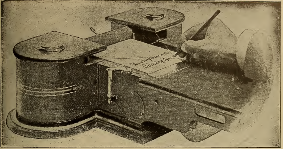
Fig. 34. THE TELAUTOGRAPH—TRANSMITTING INSTRUMENT.
